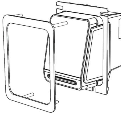
EVA Front Mounting Set Fig. 20
