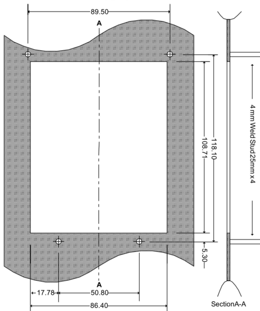
Fig. 19 – Dimensions of opening and weld studs(mm) All Dimensions [mm] +/- 0.5mm
